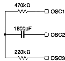
Oscillator circuit 1
