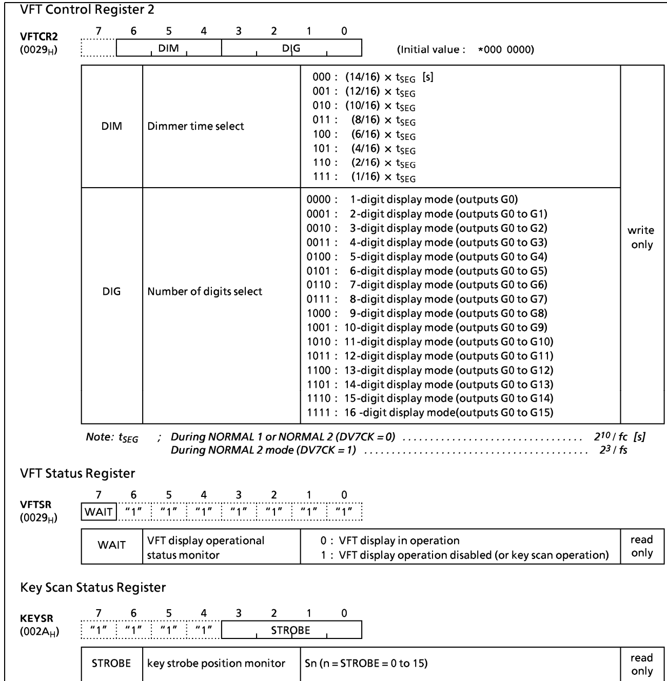
Figure 2-44 (b). VFT Control Registers/Status Registers
