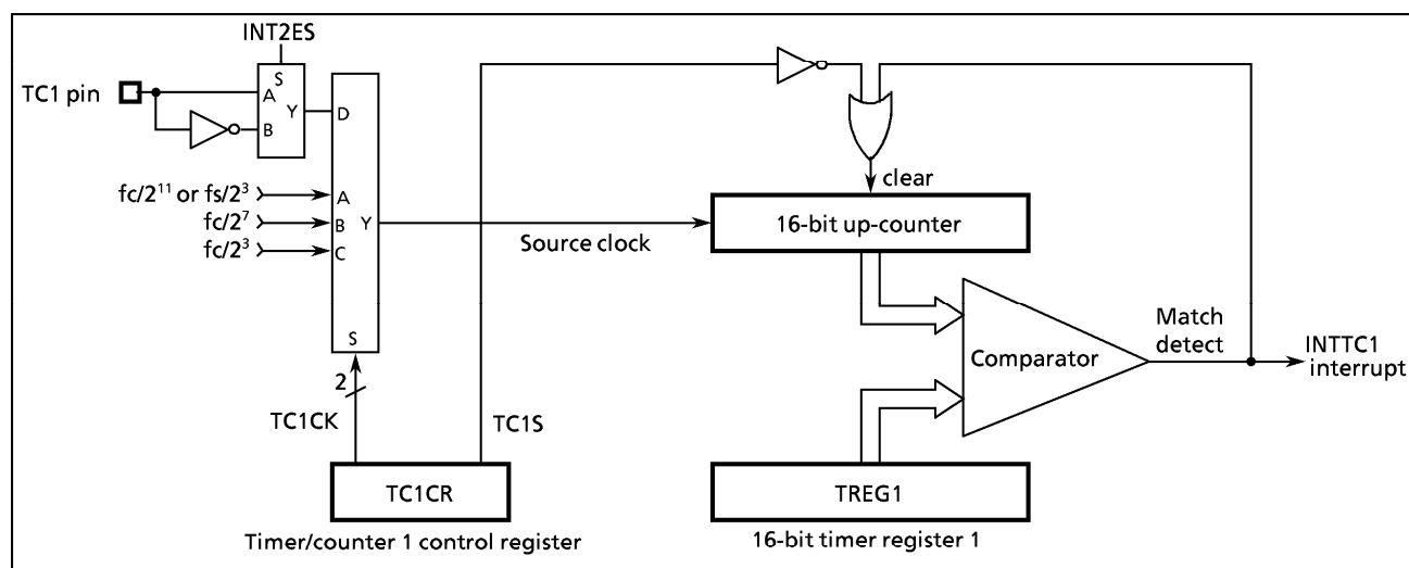
Figure 2-16. Timer/Couter 1
